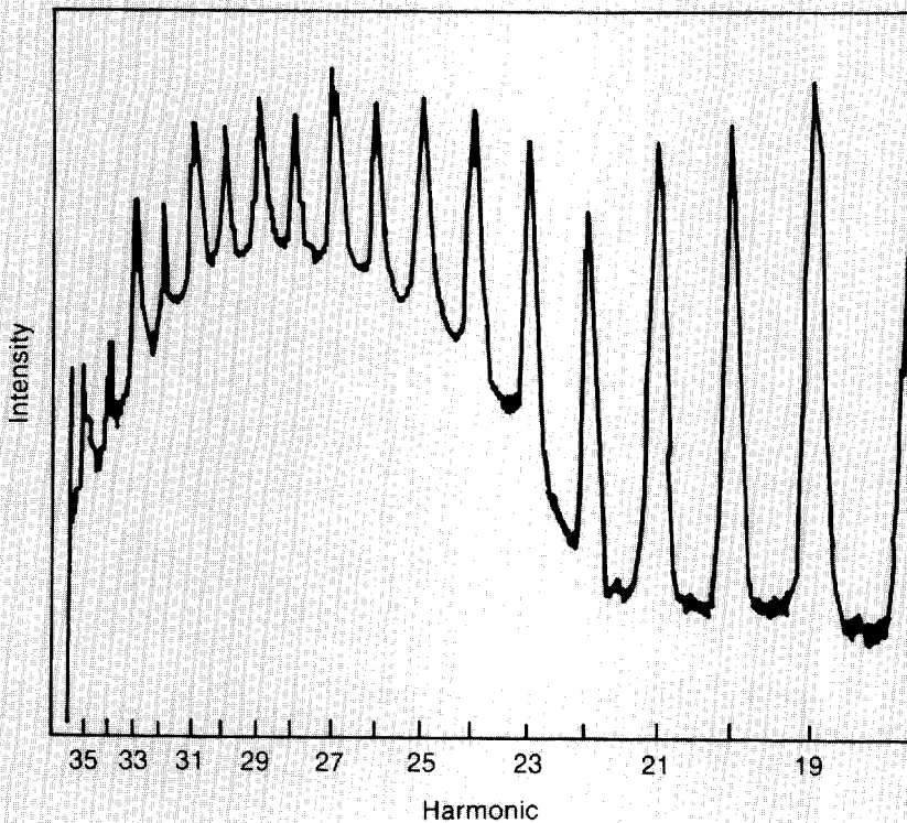
Fig. 9. Harmonics of the laser light frequency w are experimental evidence for a steepened density gradient and acceleration of electrons by wave breaking. The highest harmonic, here 35w , is a measure of the height of the upper density shelf (see Fig. 10).
