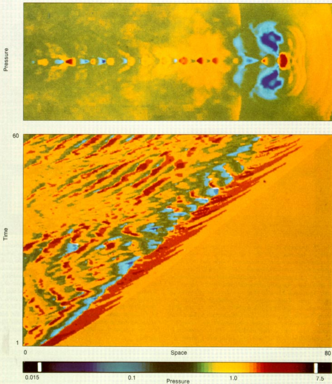
Fig. 13. Pressure fluctuations in the ( M = 3, \eta = 0.1 ) supersonic jet of Figs. 4 and 7 caused by the nonlinear growth of a reflection-mode pinch instability. Pressure values vary according to the color code. (a) The spatial pressure distribution at t = 60 shows the high-pressure knots
