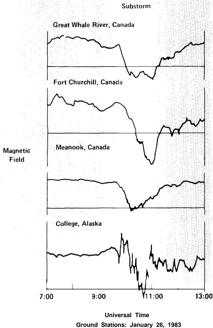
Fig. 15. Magnetic signature of an auroral substorm recorded at different ground stations on January 26, 1983. These widely separated magnetometer stations began recording, almost simultaneously at 9:45 UT, the classic “negative-bay” signature indicative of strong ionospheric current flow. The disturbance persisted for more than an hour, and the magnetic field then gradually returned to its pre-substorm values. Figures 16 and 17, respectively, show data collected during this same substorm by a satellite in geosynchronous orbit and by ISEE-3 in the distant tail.
