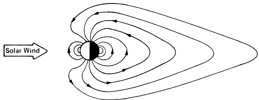
Closed Magnetosphere
