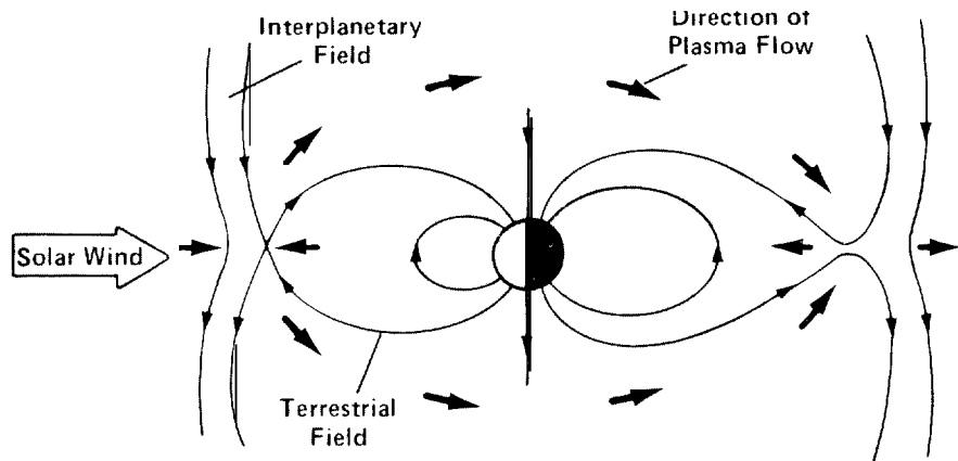
Open Magnetosphere
