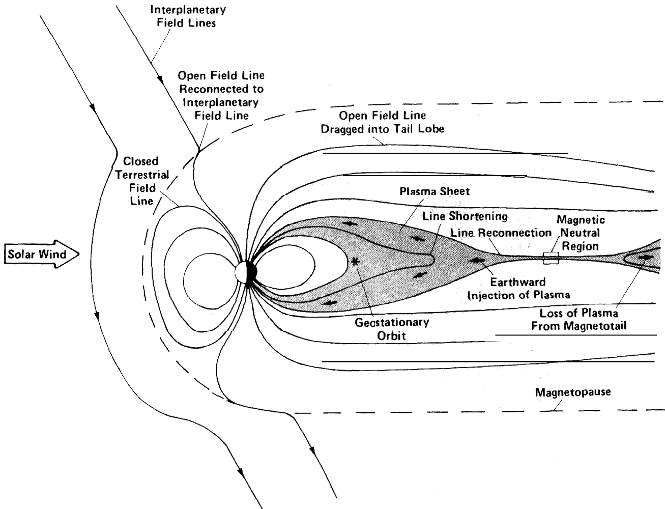
Fig. 7. Features of magnetic substorms inferred from many years of near-earth observations. Interplanetary field lines interconnect with terrestrial field lines near the front of the magnetosphere and are dragged back to form the tail lobes, carrying plasma and energy with them. Far down the tail (off the figure to the right), lobe field lines reconnect to form the plasma sheet. When the midsection of the plasma sheet becomes thin enough (due to increased magnetic pressure from the tail lobes), field lines reconnect there also, forming the
