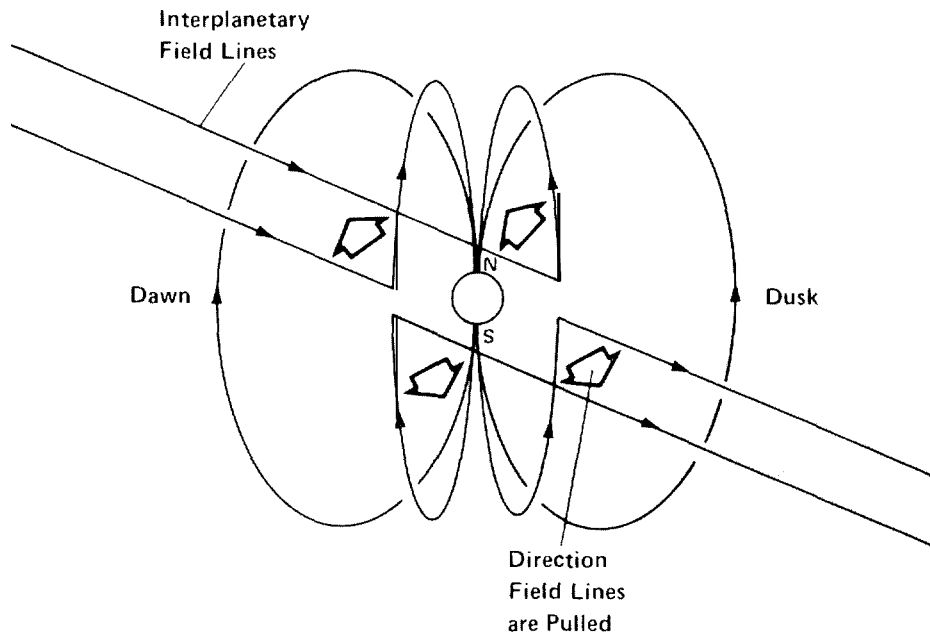
Fig. 13. Magnetic reconnection, as seen from the sun, at the dayside of the magnetosphere. The interplanetary magnet field lines shown here have their polarity directed away from the sun, have a southward component, and are reconnecting with terrestrial field lines. The reconnected field lines are dragged back into the tail lobes in the asymmetric manner indicated by the arrows. In other words, recently reconnected field lines are pulled by field tension toward opposite sides of the magnetosphere over the northern and southern polar caps. A reversal in the polarity of the interplanetary field reverses the asymmetry of this process.
