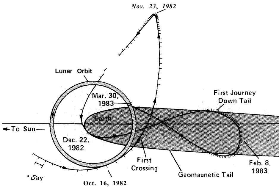
Fig. 8. The initial journeys of ISEE-3 across and down the magneto tail. The orbits, as seen from earth, are projected onto the ecliptic plane; each tic mark corresponds to one day. Lunar swing-bys were used judiciously to set up several orbits that allowed ISEE-3 to remain for long periods in the distant tail at distances up to 1,500,000 kilometers, or 230 earth radii.
