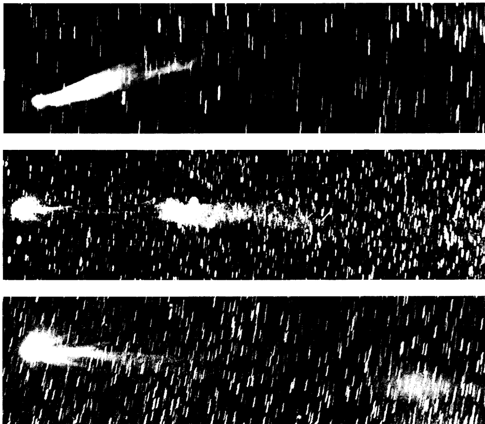
Fig. 5. Photograph (courtesy of Yerkes Observatory) of the comet Morehouse on (top 10 bottom) September 30, October 1, and October 2, 1908, showing the disconnection and drifting away of a portion of the comet's plasma tail.
