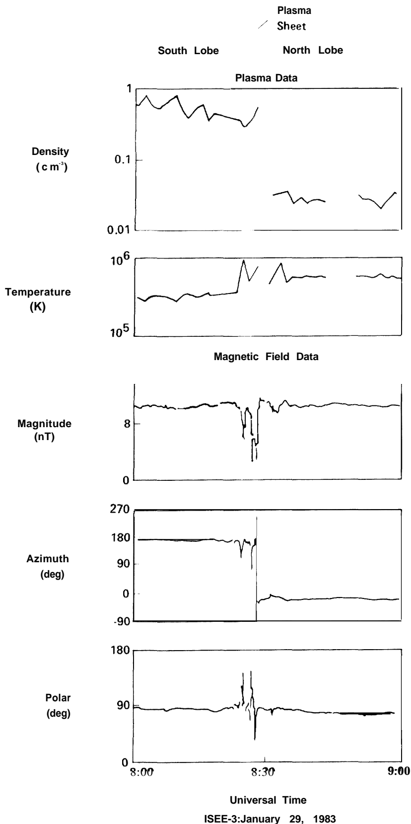
Fig. 12. These data for a traversal of the plasma sheet by ISEE-3 show a large difference between the electron densities of the north and south lobes. Such density differences are controlled by the polarity of the interplanetary magnetic field (Fig. 13) and indicate, at that point in the tail, a closed magnetopause in one lobe and an open magnetopause in the other (Fig. 14).
