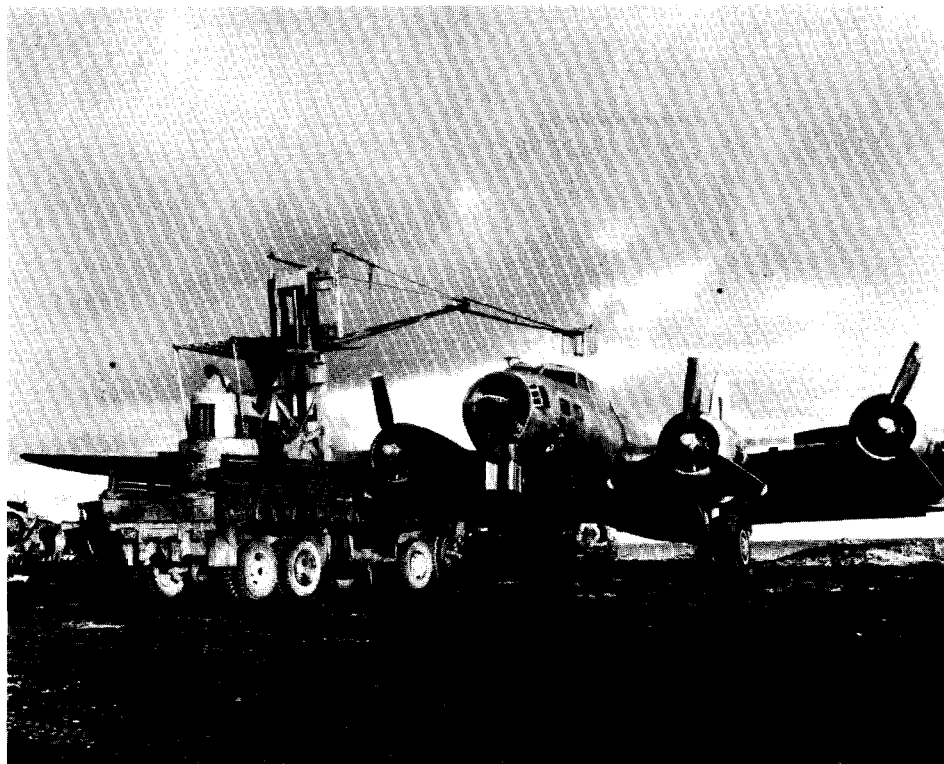
Samples of airborne debris from the Operation Crossroads tests of 1946 were gathered by drone aircraft. Shown here is a sampling unit being installed behind the cockpit of a drone B-17. The filter paper in the sampling unit was specially treated so that the debris would stick to its surface.
