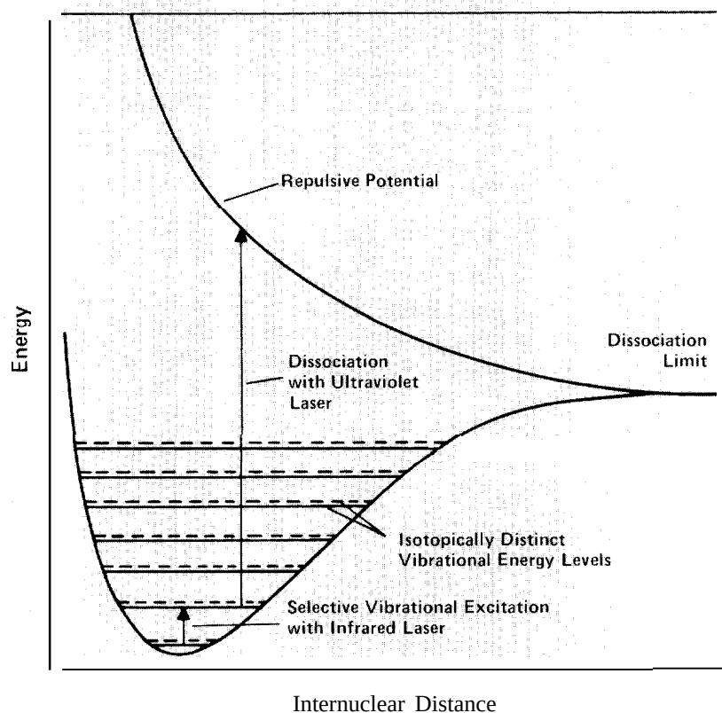
Fig. 4. In two-step photodissociation, an infrared laser selectively excites a vibrational level of one isotopic species and thereby raises molecules of that species closer to the dissociation limit. An ultraviolet laser then raises the excited molecules to an unstable electronic configuration represented by the repulsive potential. The molecule then dissociates into stable chemical fragments. (Predissociation can also occur in the ultraviolet step.)
