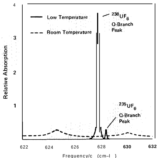
Fig. 15. The ν 3 absorption band of expansion-cooled natural-assay UF 6 exhibits narrow, distinct Q-branch peaks for 238 UF 6 and 235 UF 6 . In contrast, the room-temperature band is broad and the isotopic features are merged. (For clarity the 235 UF 6 peak is increased in height. The Q-branch peak heights for a sample containing the natural mixture of uranium isotopes are in the ratio of about 140 to 1.)
