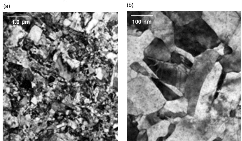
Figure 3. Nanoscale Structures in Plutonium
